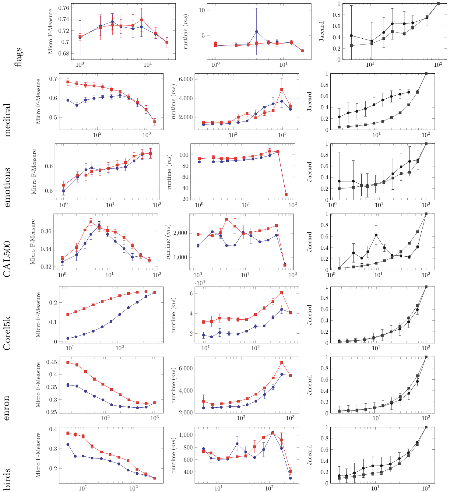
Figure 1: Global vs local feature selection comparison with J48 and average Jaccard index.
